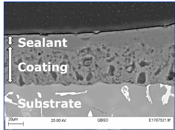
Figure 2 A cross-section of the Keronite thermal swing coating.
