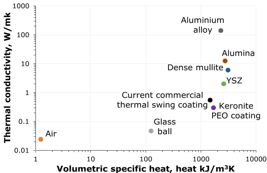
Figure 1 Thermal conductivity of various materials and thermal swing coatings.
