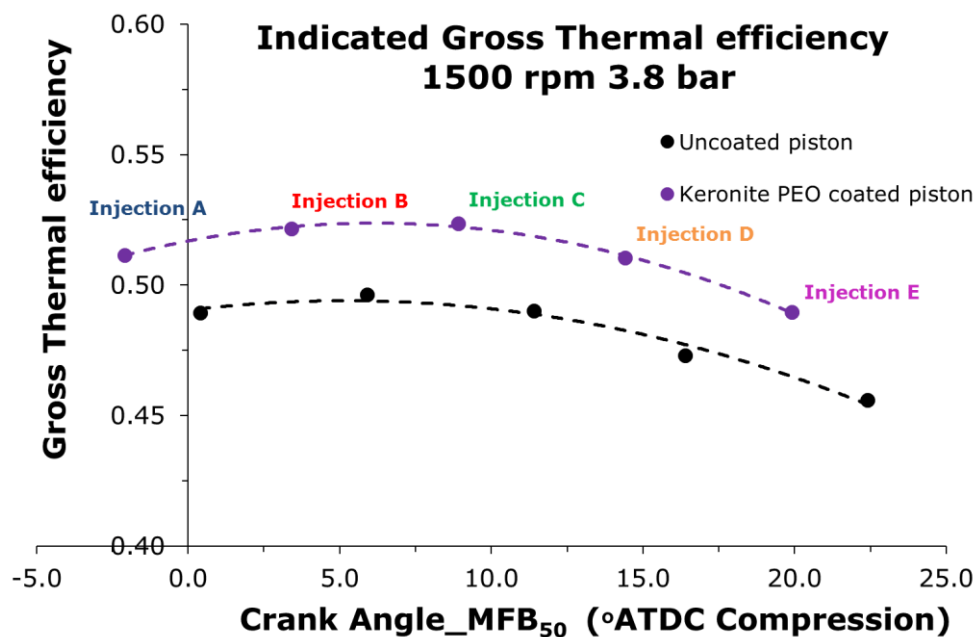
Figure 4 Indicated thermal efficiency of the Keronite PEO coated vs uncoated piston from preliminary engine tests.
