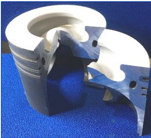
Figure 3 A photograph showing a diesel piston (Al-Si alloy) coated with a Keronite thermal swing coating on the crown and bowl regions.
